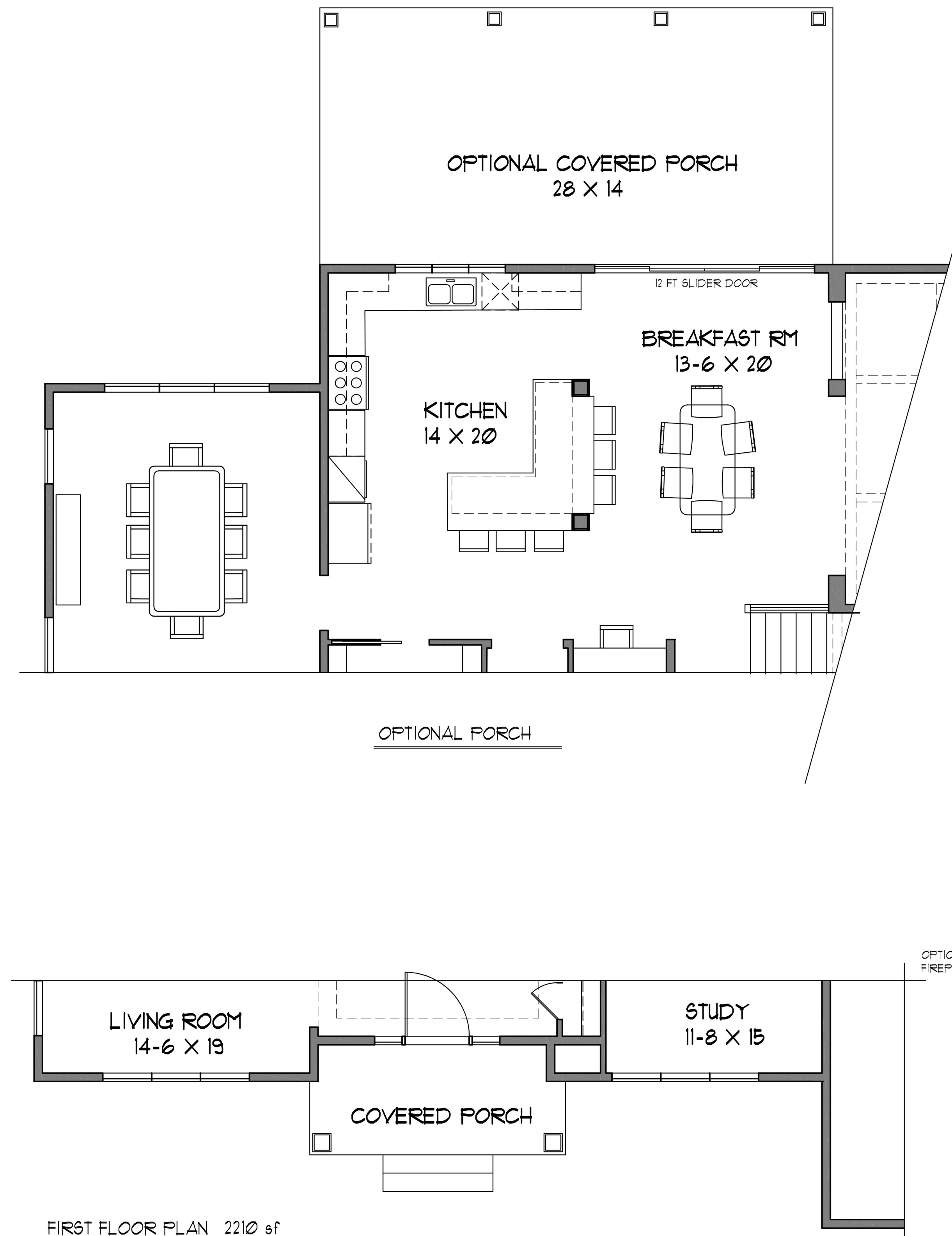
FIRST FLOOR PLAN 2210 sf TRADITIONAL
